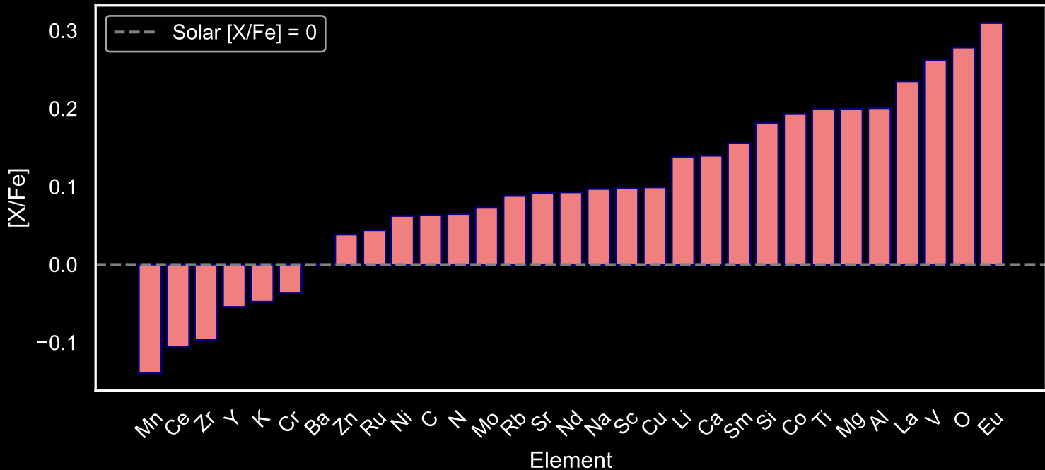
Abundance Pattern for GALAH Red Giants: Star Field [10] (N=55)
