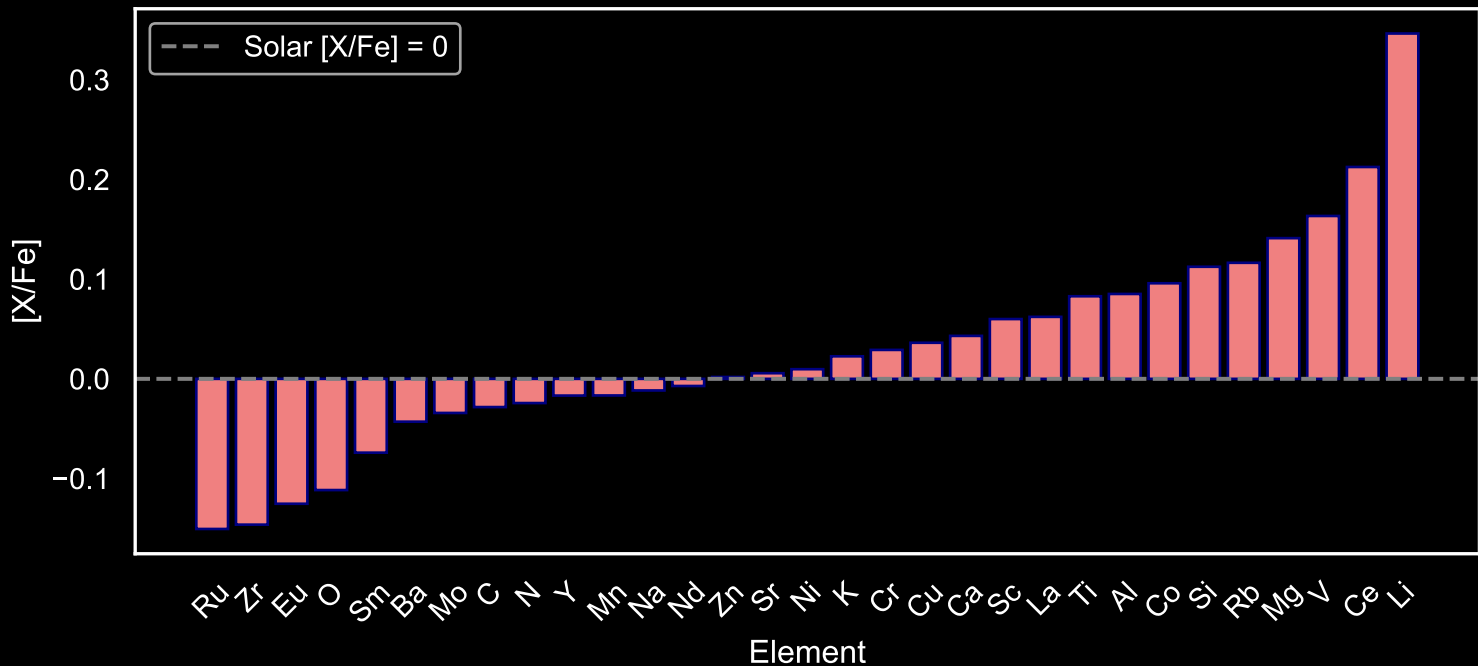
Abundance Pattern for GALAH Main Sequence Stars: Star Field [10] (N=84)
