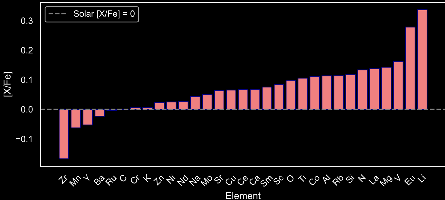
Abundance Pattern for GALAH Star Field [10] (N=198)
