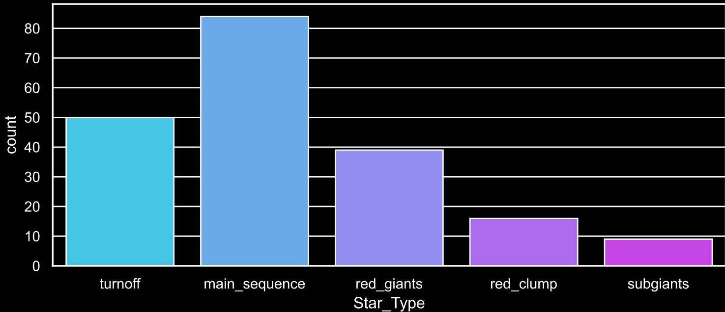
Field [10] Count plot of Star Type
